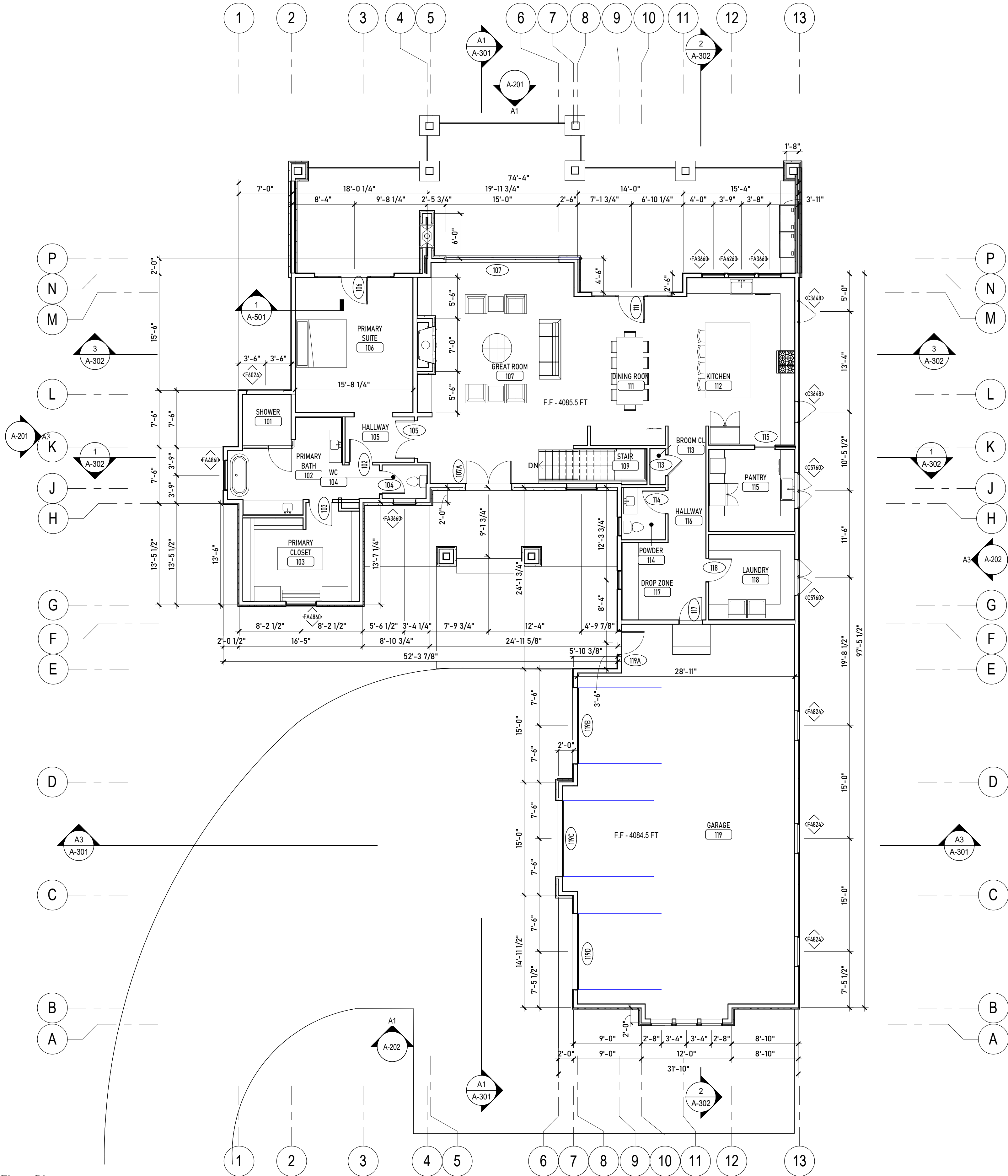
A1 First Level Floor Plan Scale: 1/8" = 1'-0"
